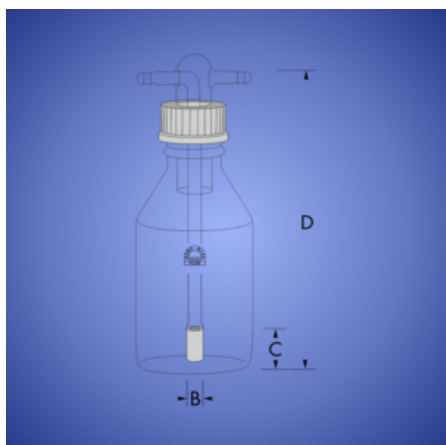
Gas washing Bottle, thread GL 45, head with filter-candle with screw cap and silicone washer
