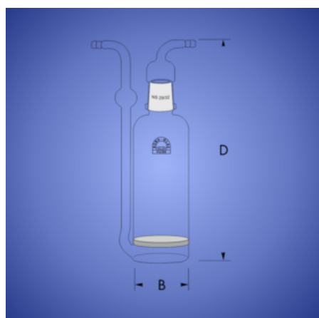
Gas Washing Bottle, sealed-in filter disc and standard joint with large filter disc and standard joint cap
