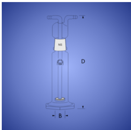
Gas Washing Bottle with standard taper joint head with filter disc
