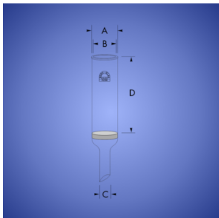
Filter Tube according to Allihn
