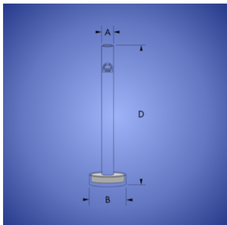
Gas Distribution Tube Type A with centered bowl
