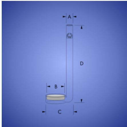
Gas Distribution Tube Type B with lateral bowl
