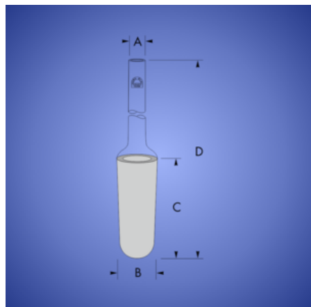
Filter-Candles, conical shape
